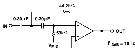
d. 2-Pole Bessel High-Pass Filter
