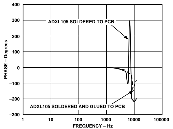
Figure 13. Phase Response
